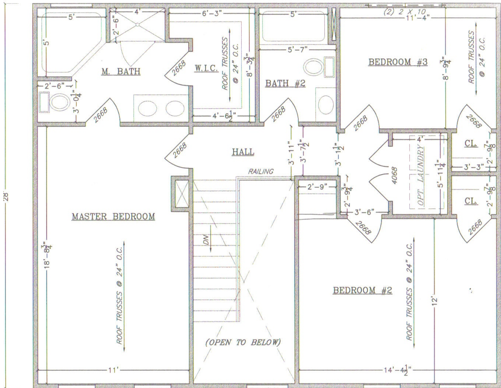
2852 ARCHED Second Floor
